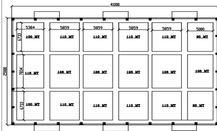
LAYOUT PLAN FOR 2000 MT WAREHOUSE
